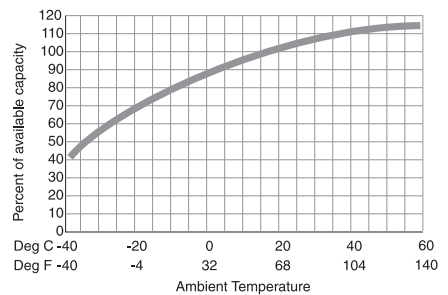
Fig. 7.8 Effect of temperature on capacity.
