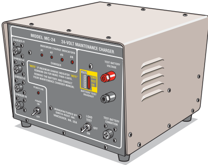
Fig. 8.1 MC-24 Maintenance Charger
