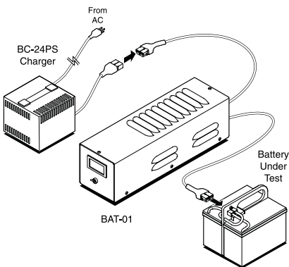
Fig. 8.3 BAT-01 Battery Analysis Tool
