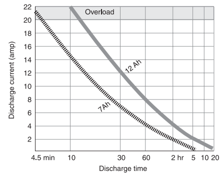
Fig. 7.6 Discharge curves for 12Ah and 7Ah batteries.
