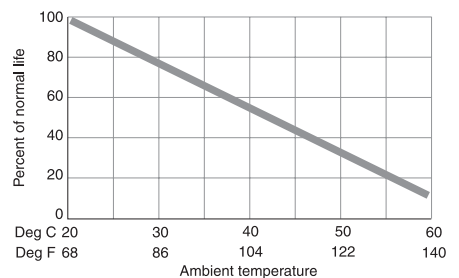
Fig. 7.7 Effect of temperature on battery life.
